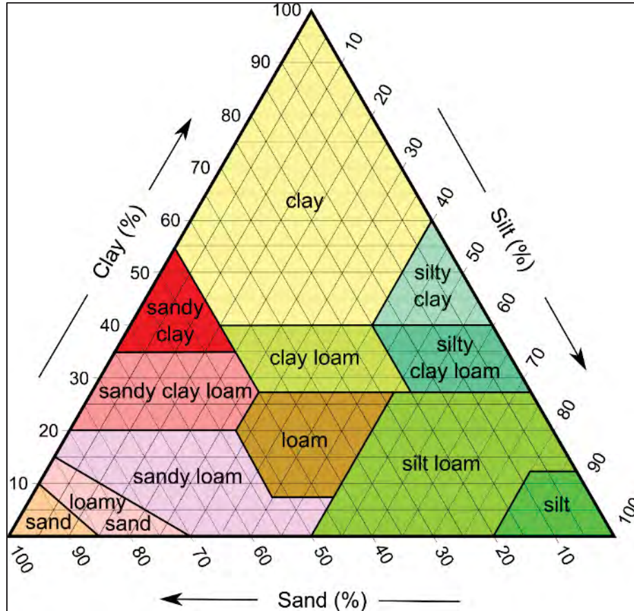
Figure 9. Soil texture triangle using percent composition of clay, silt, and sand (USDA 2016).
