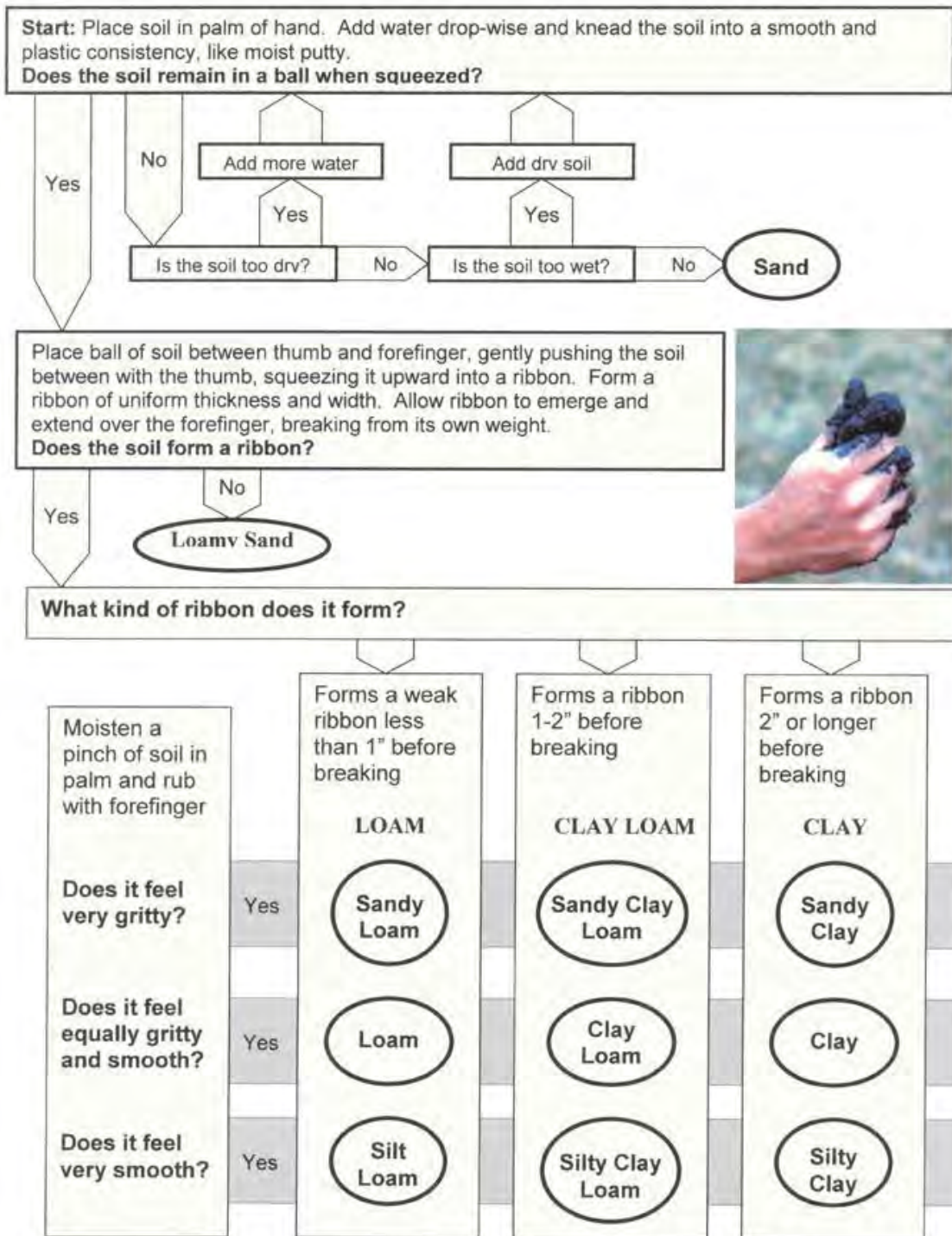
Figure 8. Soil texture by feel flowchart protocol (Whiting et al. 2015).
