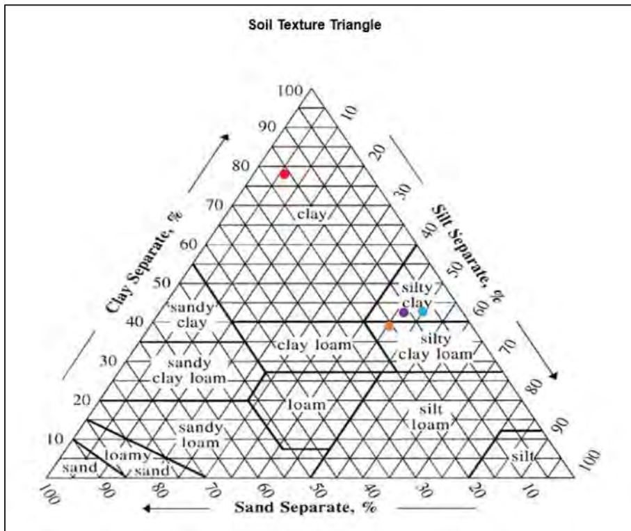
Figure 13. Soil texture by measurement results for each site overlaid onto the Soil Texture Triangle (USDA 2016).
