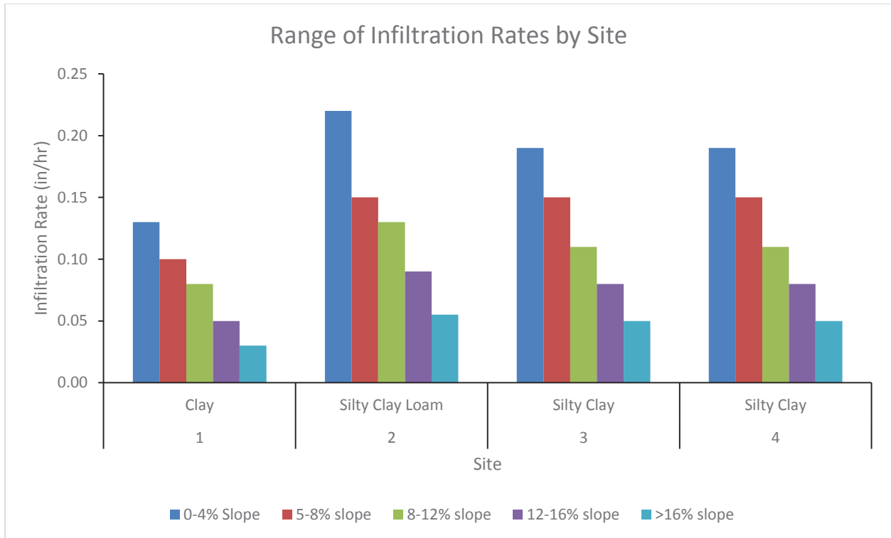
Figure 15. Range of infiltration rates by site (USDA 1990).
